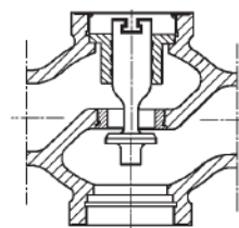
AT/S1/R (DN15)
